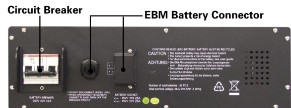
Powerware 9140 EBM (rear view)
